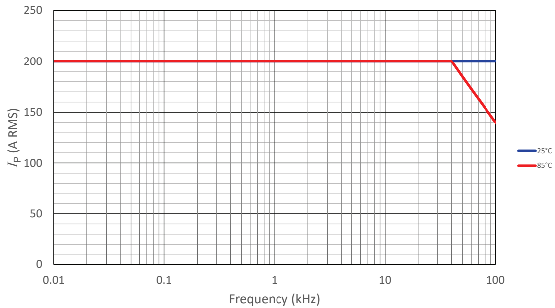
Figure 6: Derating curve
