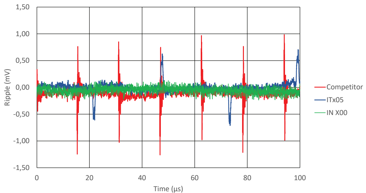
Figure 7: Ripple waveform with a 10 \Omega burden on a scope
