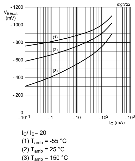
Fig. 15. BC857CQC: Base-emitter saturation voltage as a function of collector current; typical values
