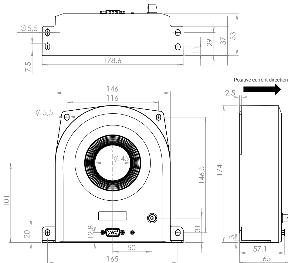
Figure 5: Dimensions of sensor head. Tolerance is 0.3 mm
