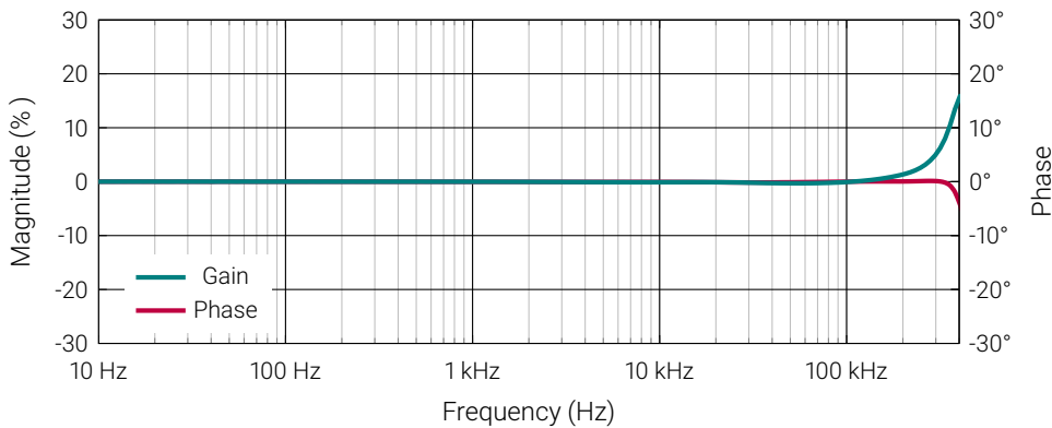
Figure 4: Frequency characteristics
