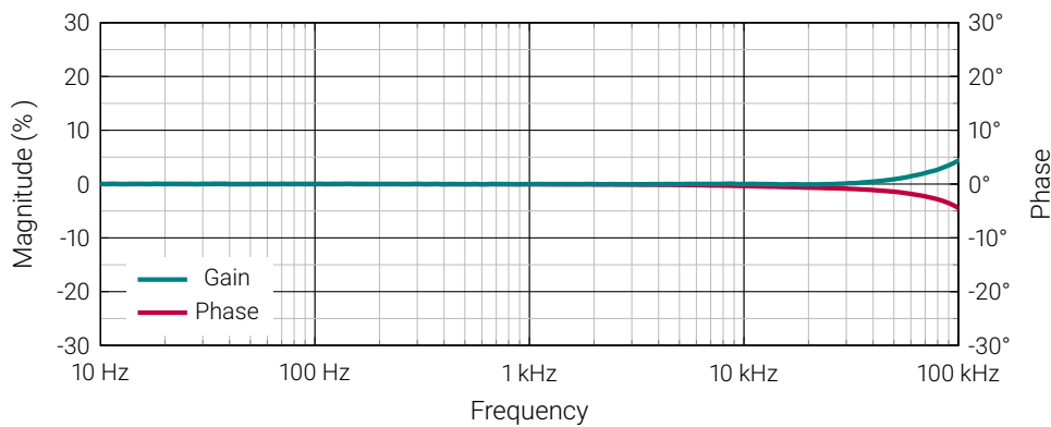
Figure 3: Frequency characteristics
