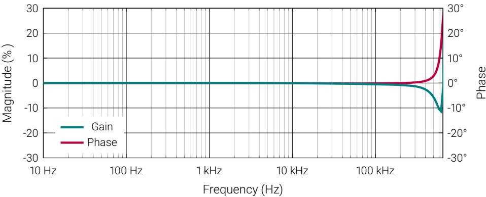
Figure 4: Frequency characteristics
