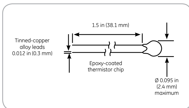
NTC Interchangeable Type DC95 dimensions
