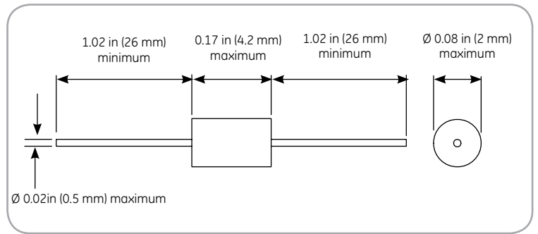
NTC Type TH dimensions
