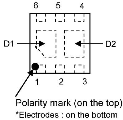
Fig. 6.2 Pin Condition(Top View)
