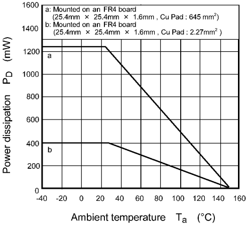
Fig. 8.14 P_D - T_a
