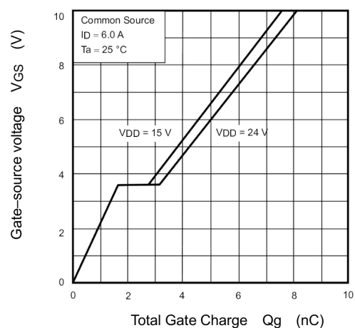
Fig. 7.10 Dynamic Input Characteristics
