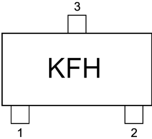
Fig. 6.1 Marking
