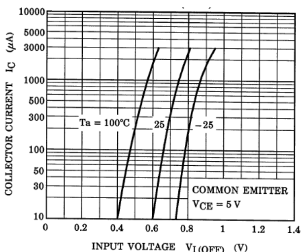
Fig. 10.12 RN1406 I_C - V_{I(OFF)}
