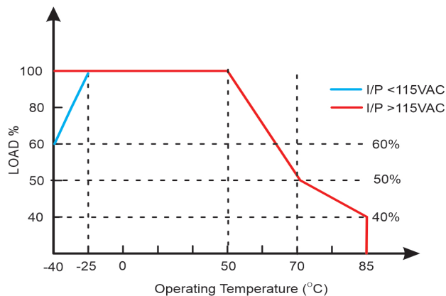
Temperature Derating Graph
