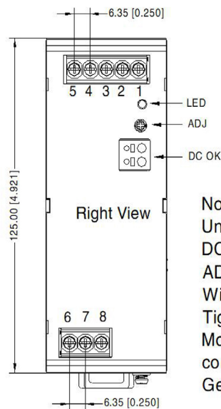
Right View
