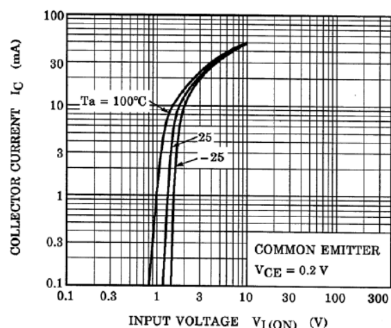
Fig. 10.2 RN1302 I_C - V_{I(ON)}
