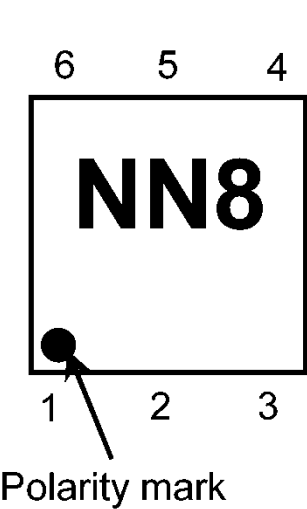
Fig. 6.1 Marking
