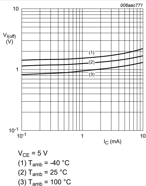
Fig. 14. PDTC114EQB-Q: Off-state input voltage as a function of collector current; typical values
