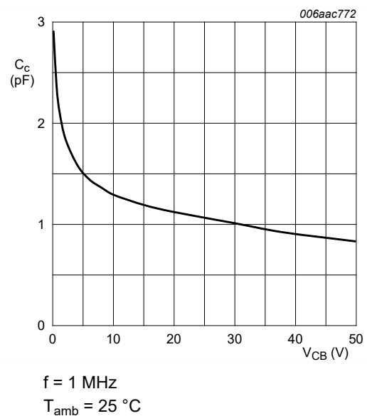
Fig. 15. PDTC114EQB-Q: Collector capacitance as a function of collector-base voltage; typical values
