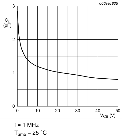
Fig. 9. PDTC143EQB-Q: Collector capacitance as a function of collector-base voltage; typical values
