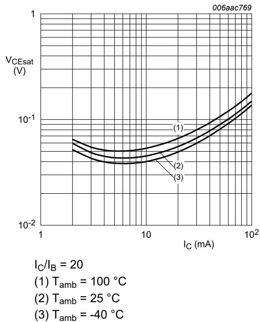
Fig. 12. PDTC114EQB-Q: Collector-emitter saturation voltage as a function of collector current; typical values
