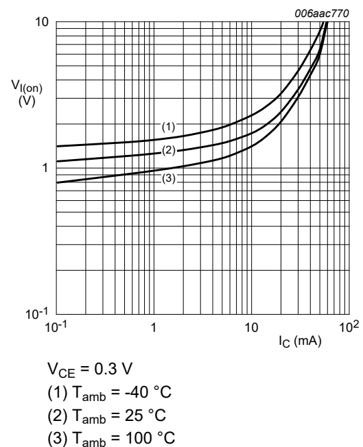
Fig. 13. PDTC114EQB-Q: On-state input voltage as a function of collector current; typical values
