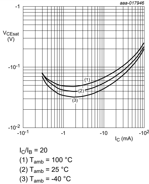
Fig. 24. PDTA144EQB-Q: Collector-emitter saturation voltage as a function of collector current; typical values
