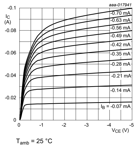
Fig. 23. PDTA144EQB-Q: Collector current as a function of collector-emitter voltage; typical values
