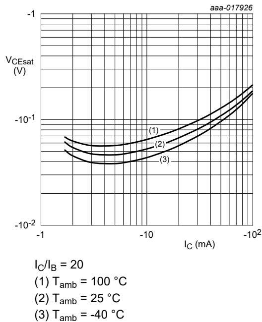
Fig. 12. PDTA114EQB-Q: Collector-emitter saturation voltage as a function of collector current; typical values
