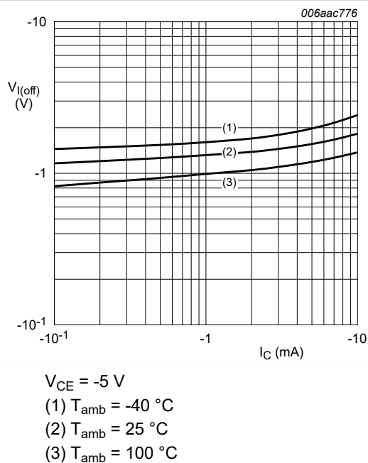
Fig. 14. PDTA114EQB-Q: Off-state input voltage as a function of collector current; typical values
