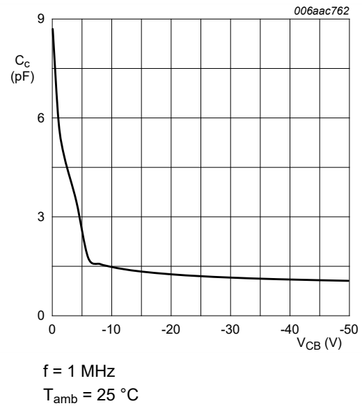
Fig. 27. PDTA144EQB-Q: Collector capacitance as a function of collector-base voltage; typical values of built-in transistor
