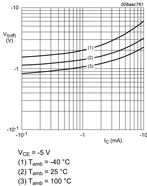
Fig. 26. PDTA144EQB-Q: Off-state input voltage as a function of collector current; typical values
