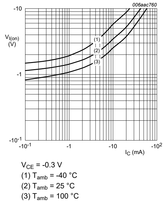
Fig. 25. PDTA144EQB-Q: On-state input voltage as a function of collector current; typical values
