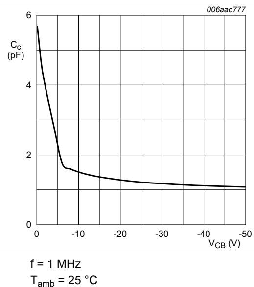
Fig. 15. PDTA114EQB-Q: Collector capacitance as a function of collector-base voltage; typical values
