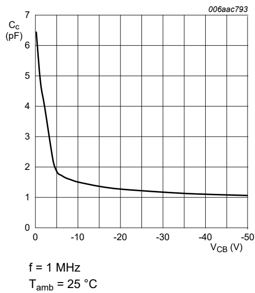
Fig. 27. PDTA114YQC-Q: Collector capacitance as a function of collector-base voltage; typical values
