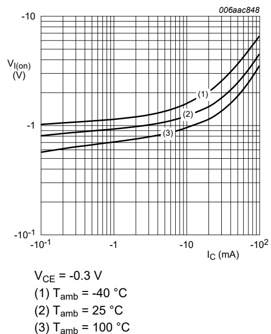
Fig. 7. PDTA143XQC-Q: On-state input voltage as a function of collector current; typical values
