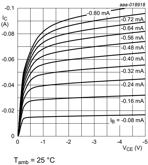
Fig. 23. PDTA114YQC-Q: Collector current as a function of collector-emitter voltage; typical values
