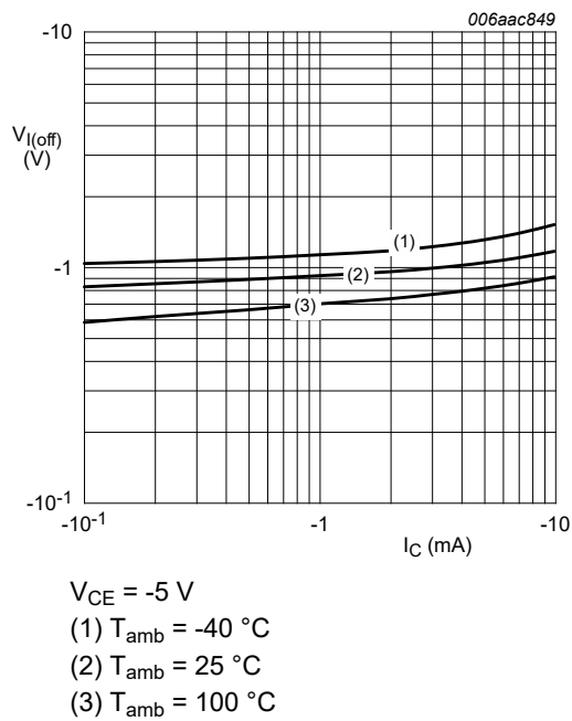
Fig. 8. PDTA143XQC-Q: Off-state input voltage as a function of collector current; typical values
