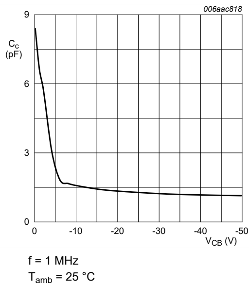
Fig. 15. PDTA123JQC-Q: Collector capacitance as a function of collector-base voltage; typical values
