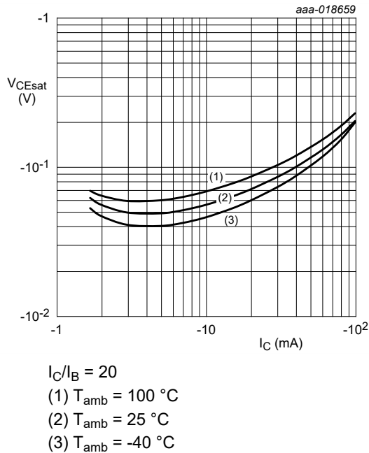
Fig. 6. PDTA143XQC-Q: Collector-emitter saturation voltage as a function of collector current; typical values
