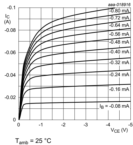
Fig. 11. PDTA123JQC-Q: Collector current as a function of collector-emitter voltage; typical values
