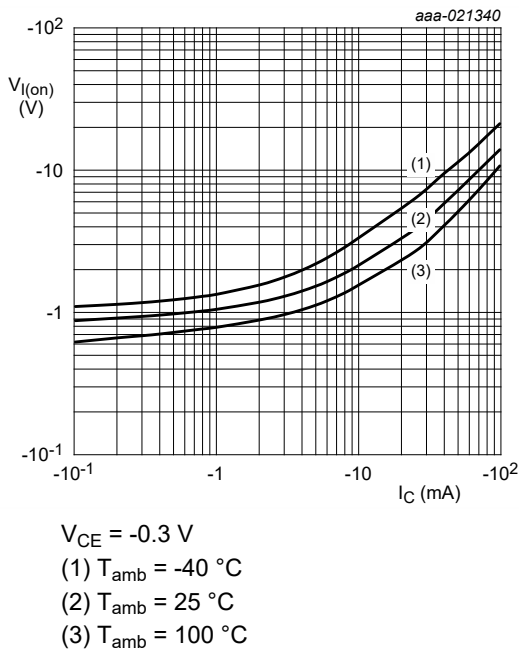
Fig. 31. PDTA124XQB-Q: On-state input voltage as a function of collector current; typical values
