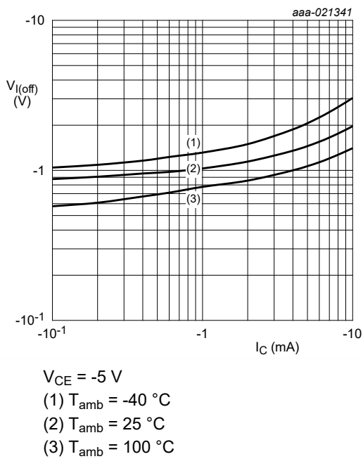
Fig. 32. PDTA124XQB-Q: Off-state input voltage as a function of collector current; typical values
