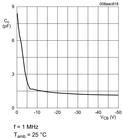
Fig. 15. PDTA123JQB-Q: Collector capacitance as a function of collector-base voltage; typical values
