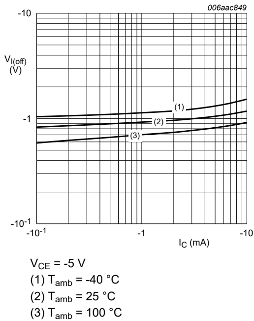
Fig. 8. PDTA143XQB-Q: Off-state input voltage as a function of collector current; typical values
