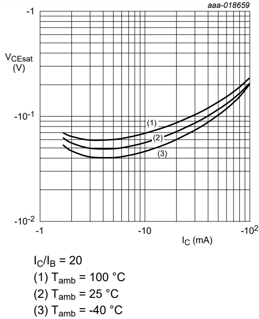
Fig. 6. PDTA143XQB-Q: Collector-emitter saturation voltage as a function of collector current; typical values
