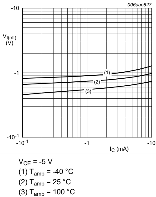
Fig. 20. PDTA143ZQB-Q: Off-state input voltage as a function of collector current; typical values
