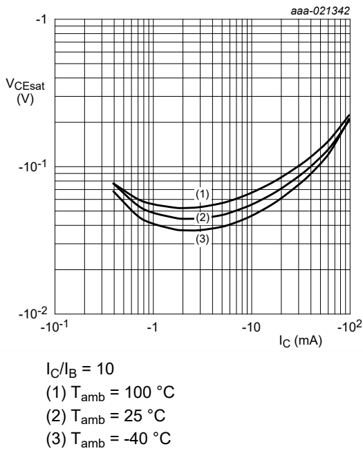
Fig. 30. PDTA124XQB-Q: Collector-emitter saturation voltage as a function of collector current; typical values
