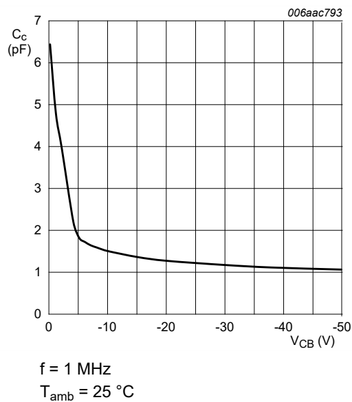
Fig. 27. PDTA114YQB-Q: Collector capacitance as a function of collector-base voltage; typical values
