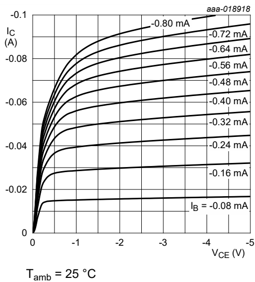
Fig. 23. PDTA114YQB-Q: Collector current as a function of collector-emitter voltage; typical values
