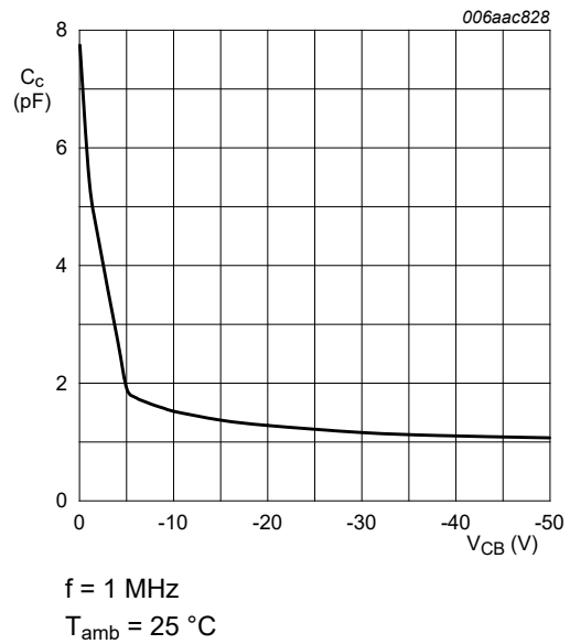
Fig. 21. PDTA143ZQB-Q: Collector capacitance as a function of collector-base voltage; typical values
