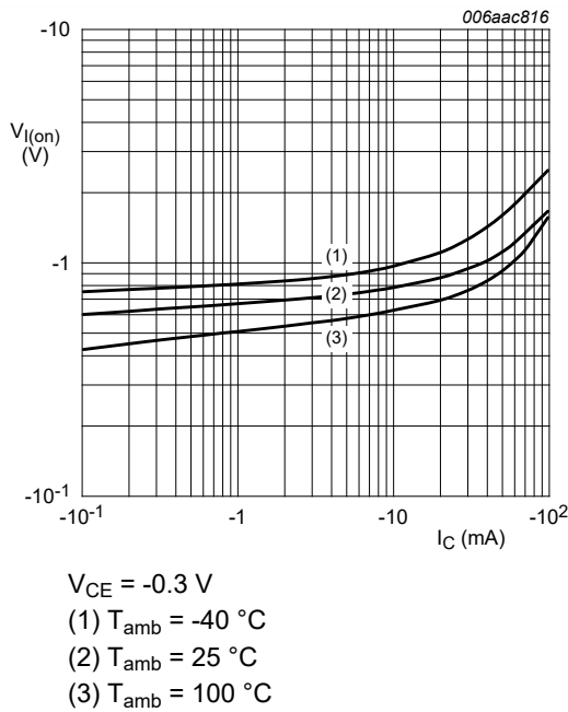
Fig. 13. PDTA123JQB-Q: On-state input voltage as a function of collector current; typical values
