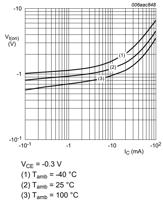
Fig. 7. PDTA143XQB-Q: On-state input voltage as a function of collector current; typical values
