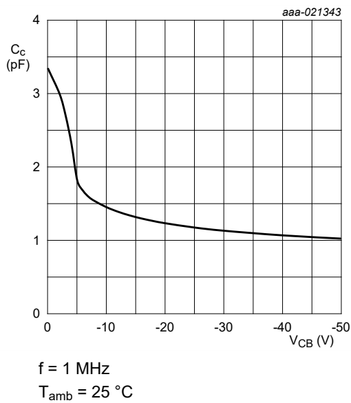
Fig. 33. PDTA124XQB-Q: Collector capacitance as a function of collector-base voltage; typical values
