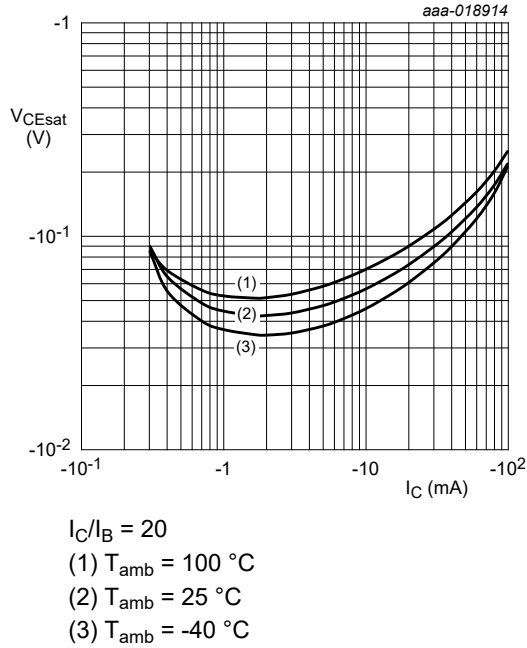
Fig. 18. PDTA143ZQB-Q: Collector-emitter saturation voltage as a function of collector current; typical values
