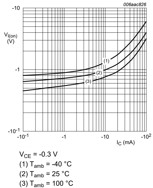
Fig. 19. PDTA143ZQB-Q: On-state input voltage as a function of collector current; typical values
