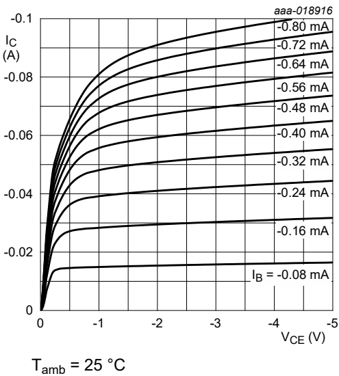
Fig. 11. PDTA123JQB-Q: Collector current as a function of collector-emitter voltage; typical values
