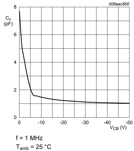
Fig. 9. PDTA143XQB-Q: Collector capacitance as a function of collector-base voltage; typical values
