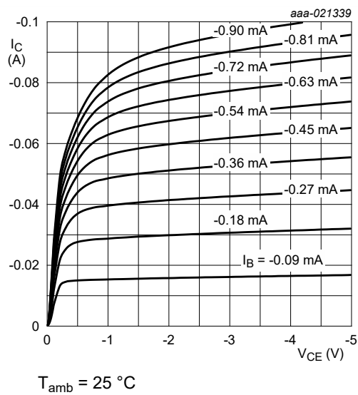
Fig. 29. PDTA124XQB-Q: Collector current as a function of collector-emitter voltage; typical values
