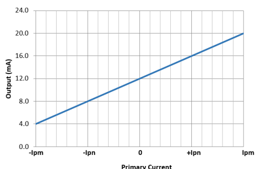
Figure 1: Transfer characteristics
