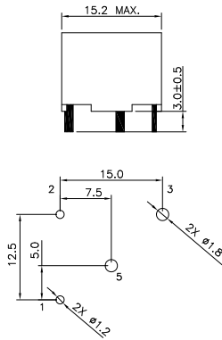
SUGGESTED LAND PATTERN
