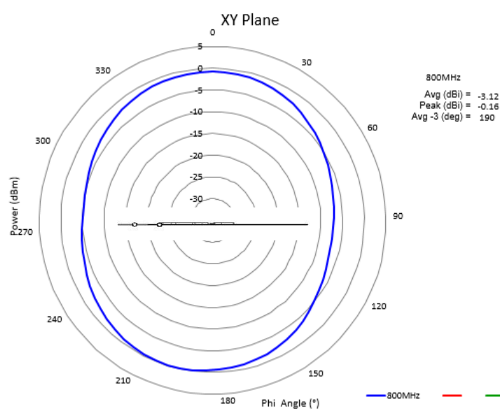
Horizontal Plane
