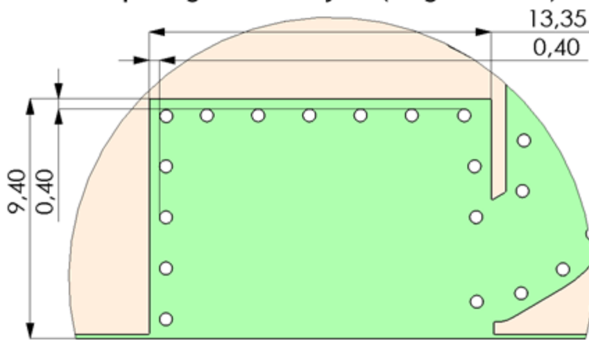
DETAIL C
