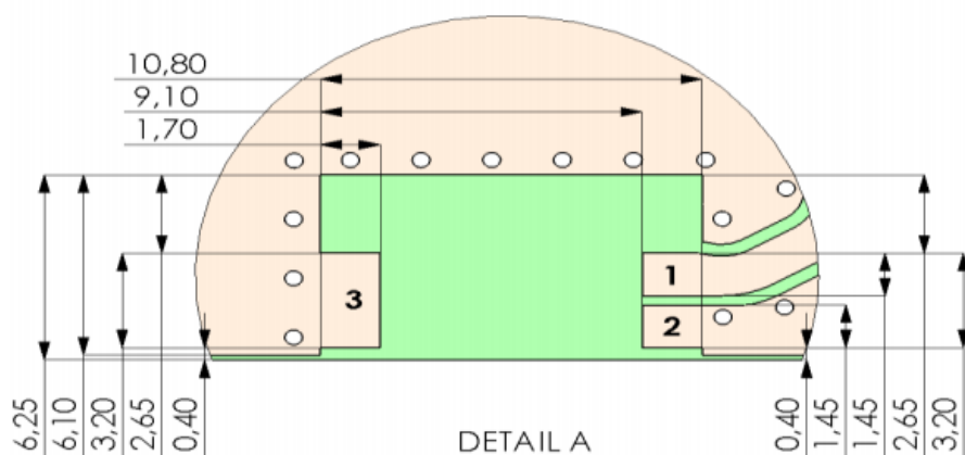
Pad dimensions on PWB layout
