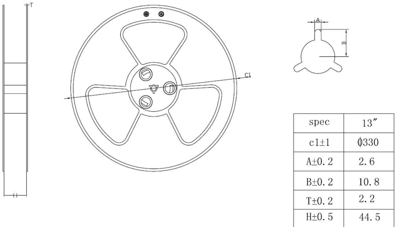
Figure 10.2. Reel Dimensions
