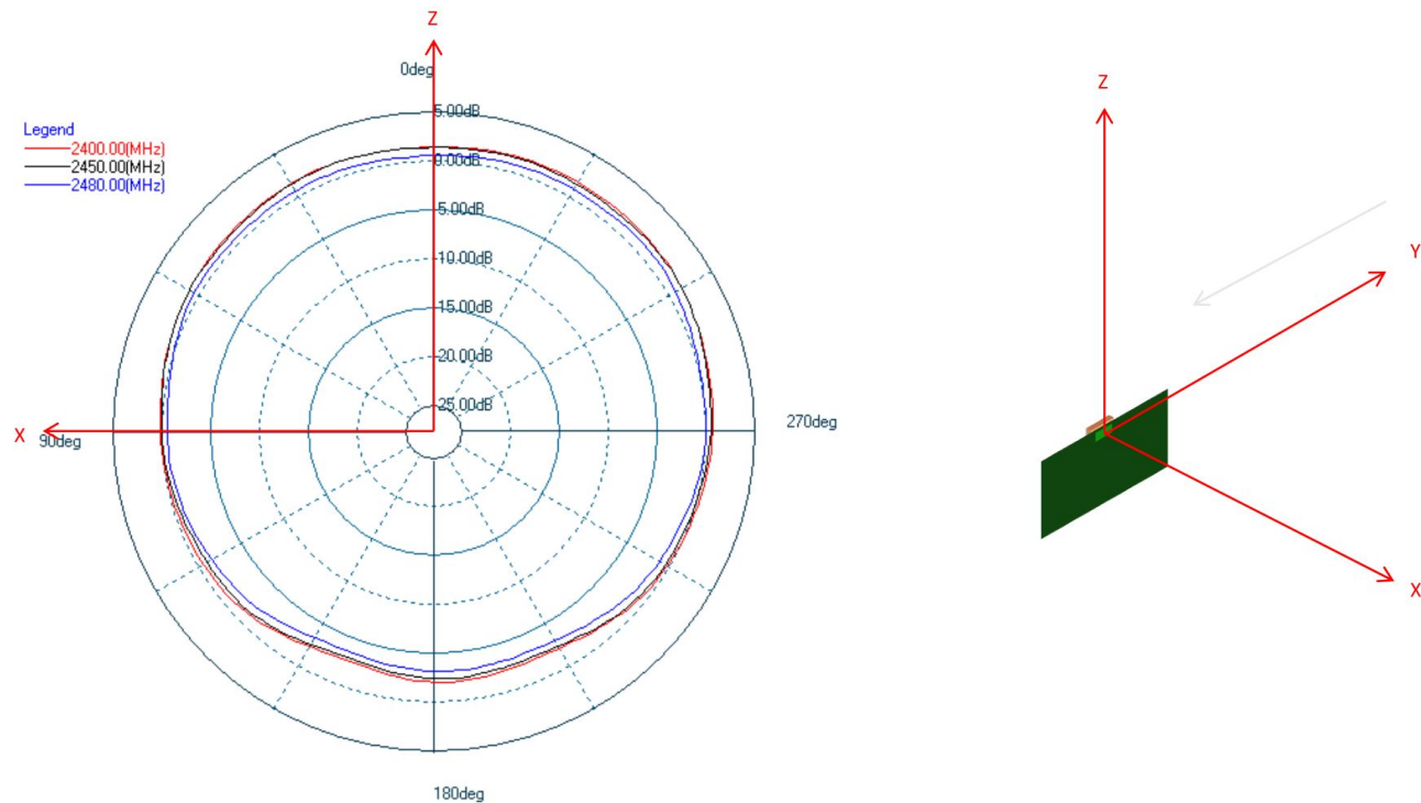
Figure 4.3. Typical 2D Antenna Radiation Patterns - \Phi = 0^\circ (Side View) Gain (dBi)
