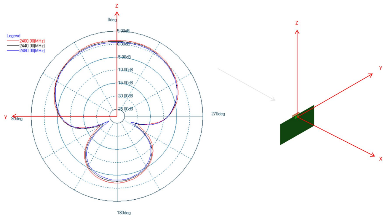
Figure 4.4. Typical 2D Antenna Radiation Patterns - \Phi = 90^\circ (Top View) Gain (dBi)
