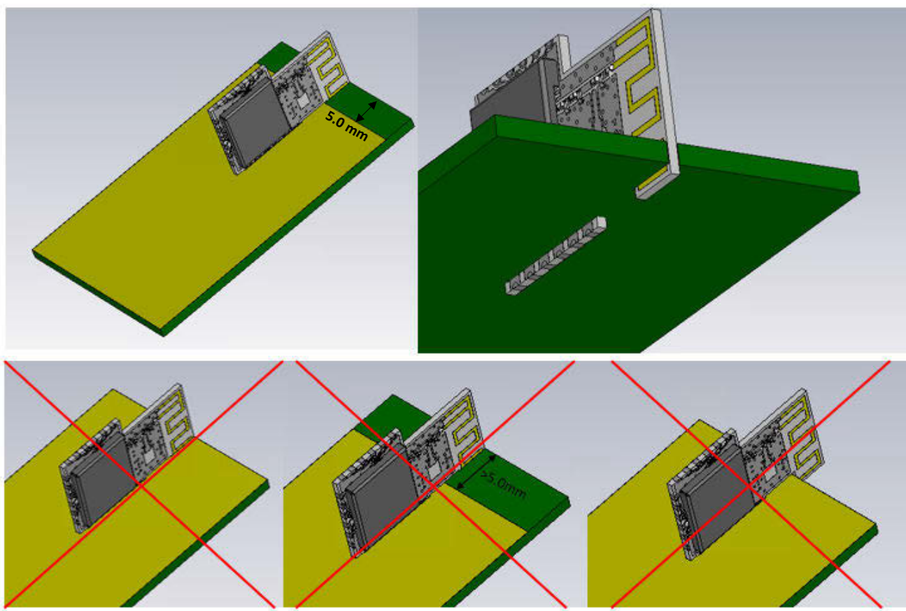
Figure 7.3. Vertical Mounting
