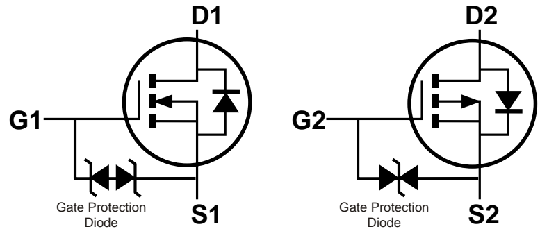
Internal Schematic
