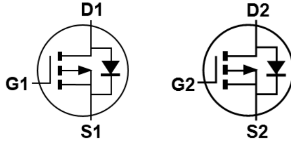
Internal Schematic
