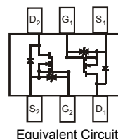
Equivalent Circuit
