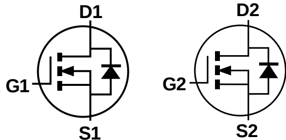
Internal Schematic
