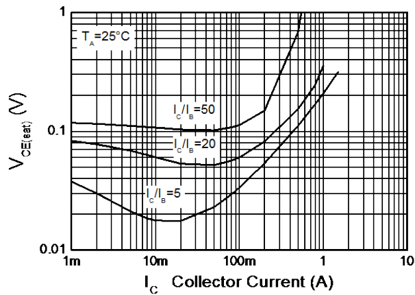
Fig 7: Typical Collector-Emitter Saturation Voltage vs Collector Current
