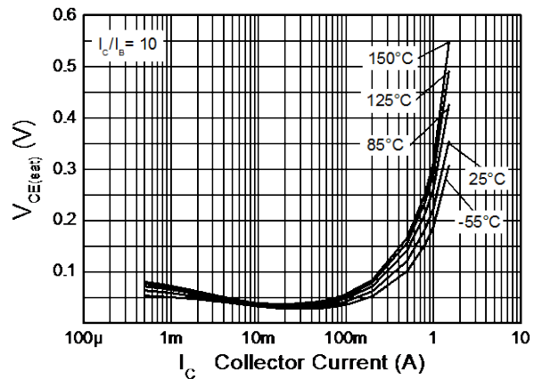
Fig 6: Typical Collector-Emitter Saturation Voltage vs Collector Current
