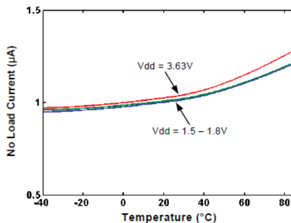
Total Supply Current vs Operating Temperature Range (Core+LVCMOS Output Driver, No Load)
