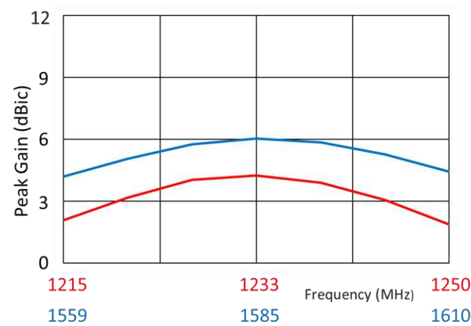
Peak Gain
