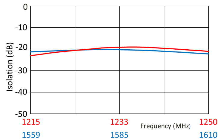
Isolation
