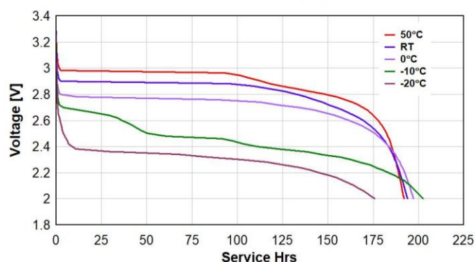
Temperature Discharge 5000 \Omega Continuous to 2V
