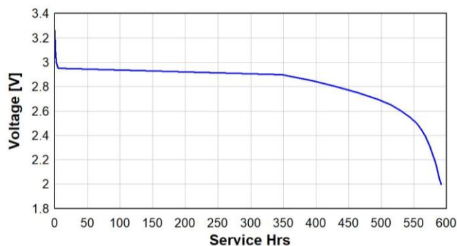
Continuous Discharge 15k \Omega continuous until 2V
