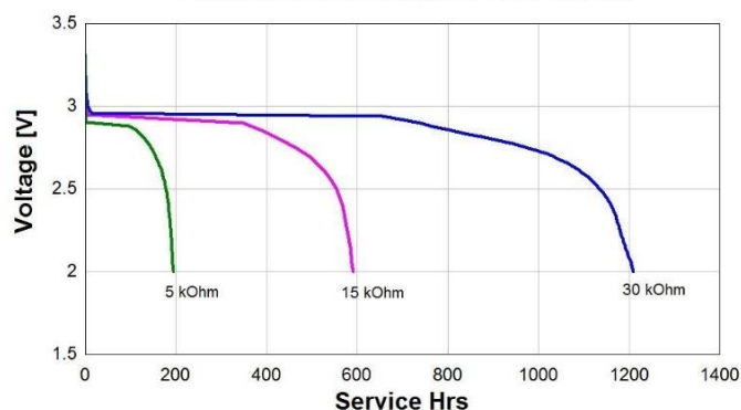
Continuous Discharge to 2.0V cut-off
