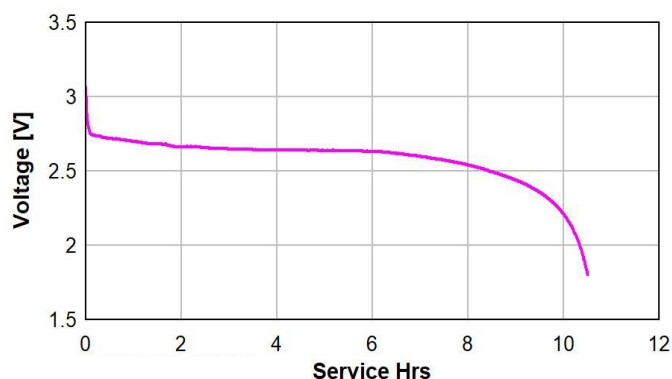
Pulse Discharge 10 mA 5s/m, 24h/d 1.8V
