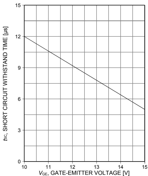
Figure 20. Short circuit withstand time as a function of gate-emitter voltage ( V_{CE} \leq 400V , start at T_J \leq 150^\circ C )
