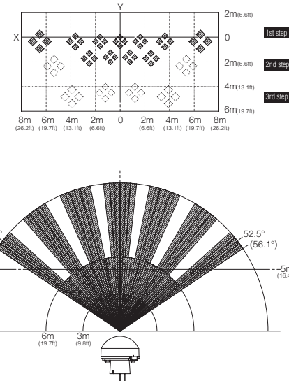
X-Y cross section at 5m (16.4ft)
