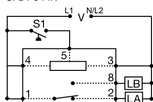
SPDT 8-PIN
