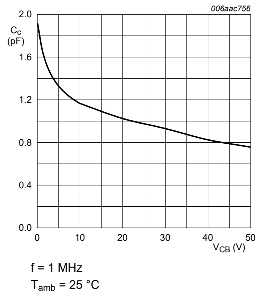
Fig. 27. PDTC144EQB: Collector capacitance as a function of collector-base voltage; typical values
