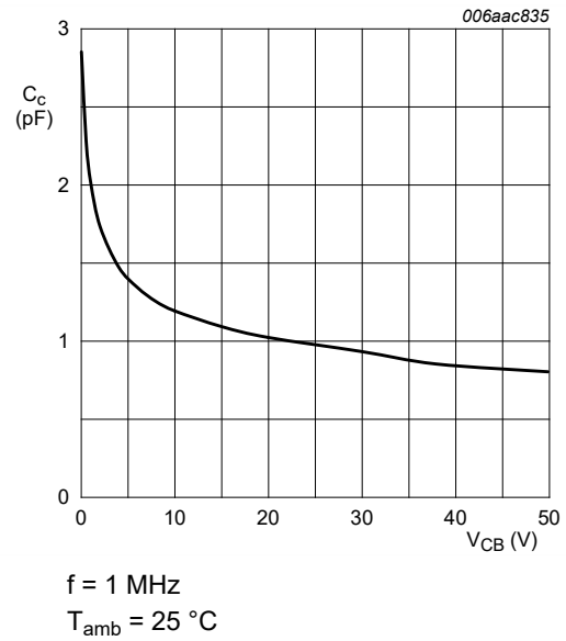
Fig. 9. PDTC143EQB: Collector capacitance as a function of collector-base voltage; typical values
