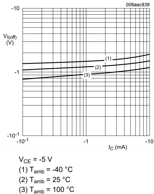
Fig. 8. PDTA143EQB: Off-state input voltage as a function of collector current; typical values
