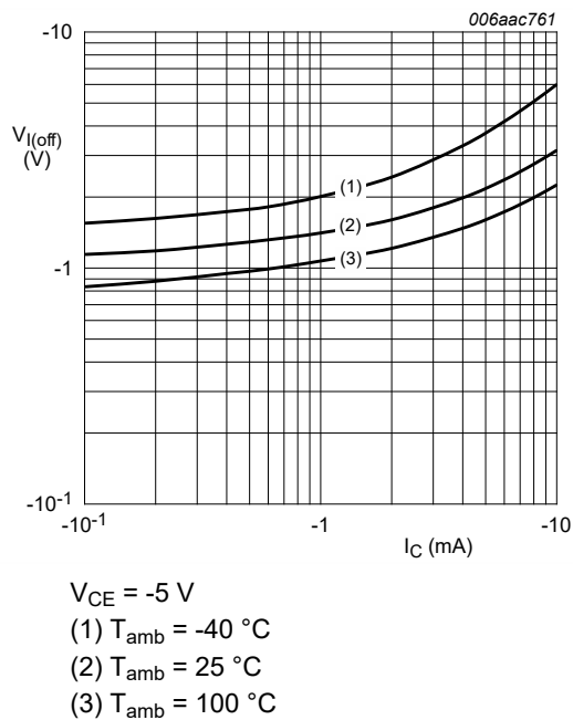
Fig. 26. PDTA144EQB: Off-state input voltage as a function of collector current; typical values
