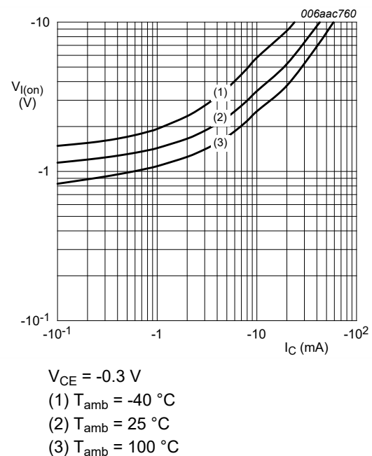
Fig. 25. PDTA144EQB: On-state input voltage as a function of collector current; typical values
