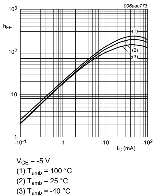
Fig. 10. PDTA114EQB: DC current gain as a function of collector current; typical values
