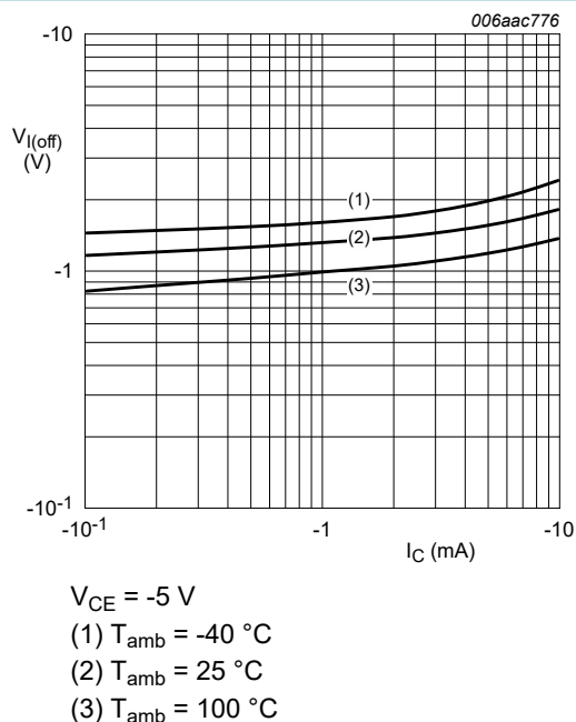
Fig. 14. PDTA114EQB: Off-state input voltage as a function of collector current; typical values
