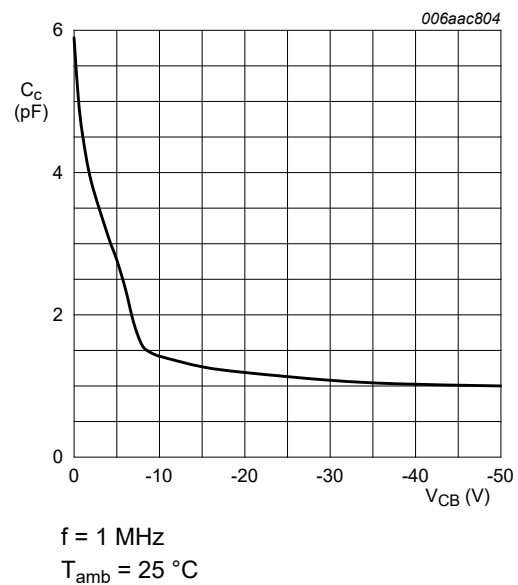
Fig. 21. PDTA124EQB: Collector capacitance as a function of collector-base voltage; typical values
