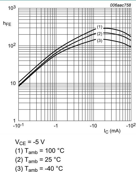
Fig. 22. PDTA144EQB: DC current gain as a function of collector current; typical values
