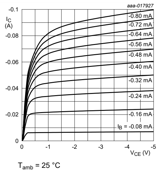
Fig. 11. PDTA114EQB: Collector current as a function of collector-emitter voltage; typical values
