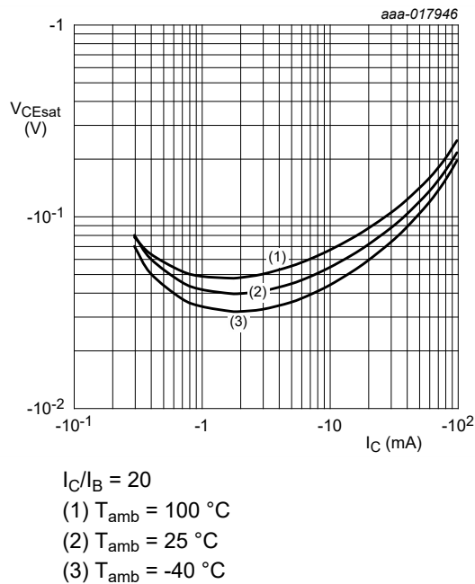
Fig. 24. PDTA144EQB: Collector-emitter saturation voltage as a function of collector current; typical values
