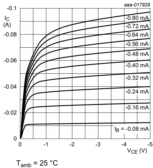
Fig. 17. PDTA124EQB: Collector current as a function of collector-emitter voltage; typical values
