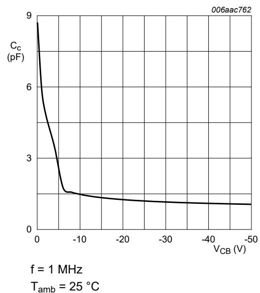
Fig. 27. PDTA144EQB: Collector capacitance as a function of collector-base voltage; typical values of built-in transistor
