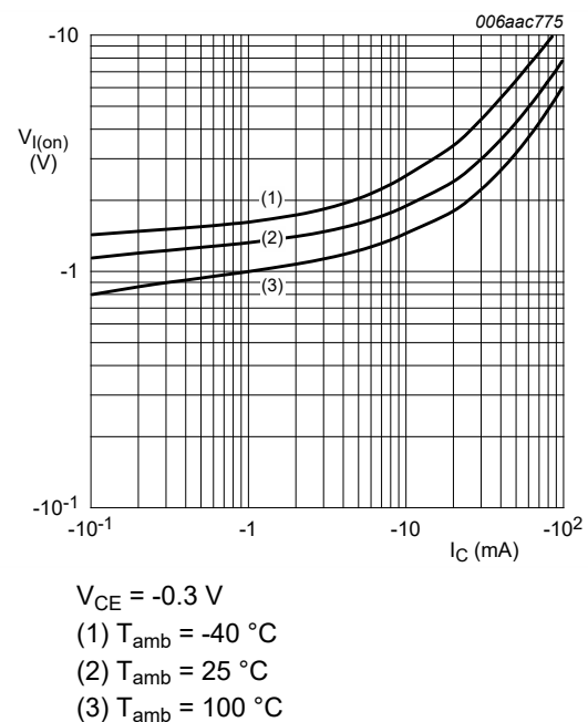
Fig. 13. PDTA114EQB: On-state input voltage as a function of collector current; typical values
