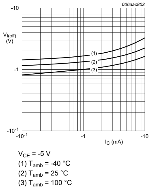
Fig. 20. PDTA124EQB: Off-state input voltage as a function of collector current; typical values
