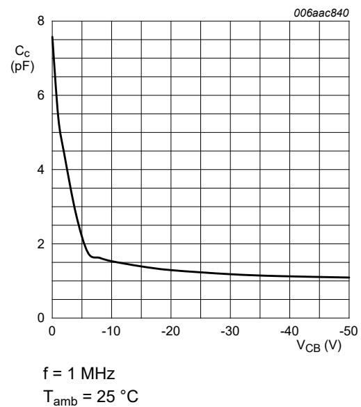
Fig. 9. PDTA143EQB: Collector capacitance as a function of collector-base voltage; typical values
