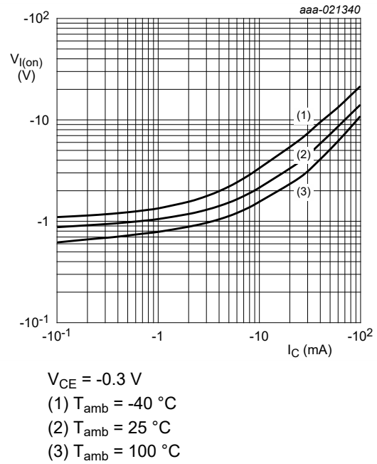
Fig. 31. PDTA124XQB: On-state input voltage as a function of collector current; typical values
