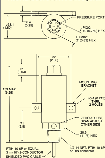
PX02/PXM02 Barometer with Mounting Bracket
