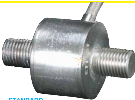
STANDARD LC202-10K, shown close to actual size.
