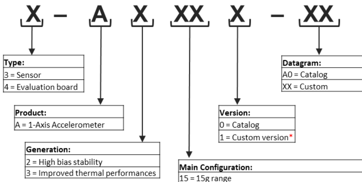
Figure 28: Ordering information
