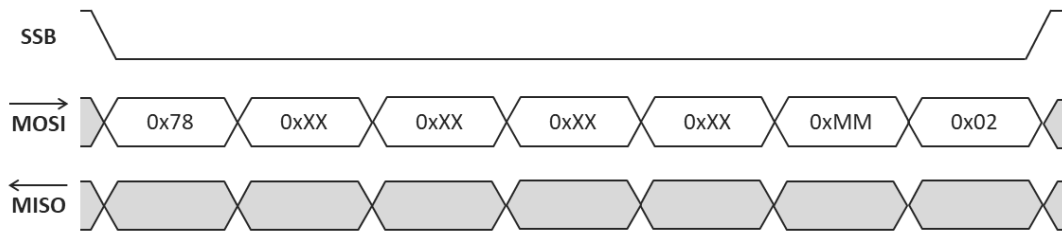
Figure 22: Sequence of instructions to WRITE '0XXXXXXXX' to address '0xMM' of the system registers
