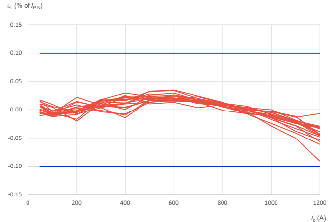
Linearity error (% of I_{PN} ) @ 25 °C
