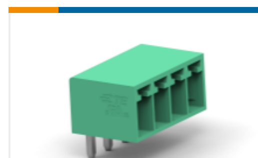
TE Model / Part #1-2350514-4 14POS TB HDR 90 DEG, PITCH 3.5 & TL 3.5mm
