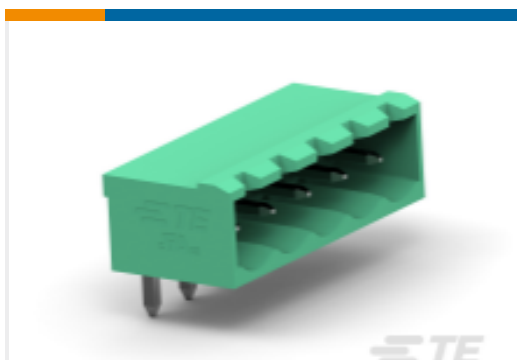
TE Model / Part #2350513-5 5POS TB HDR 90 DEG, PITCH 5.0 & TL 4.5mm
