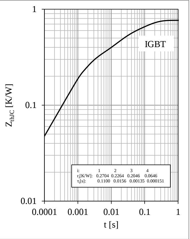
Fig 6. IGBT-inverter Transient Thermal Impedance
