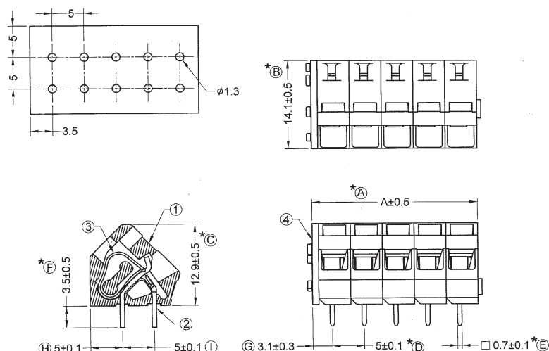
PCB Layout
